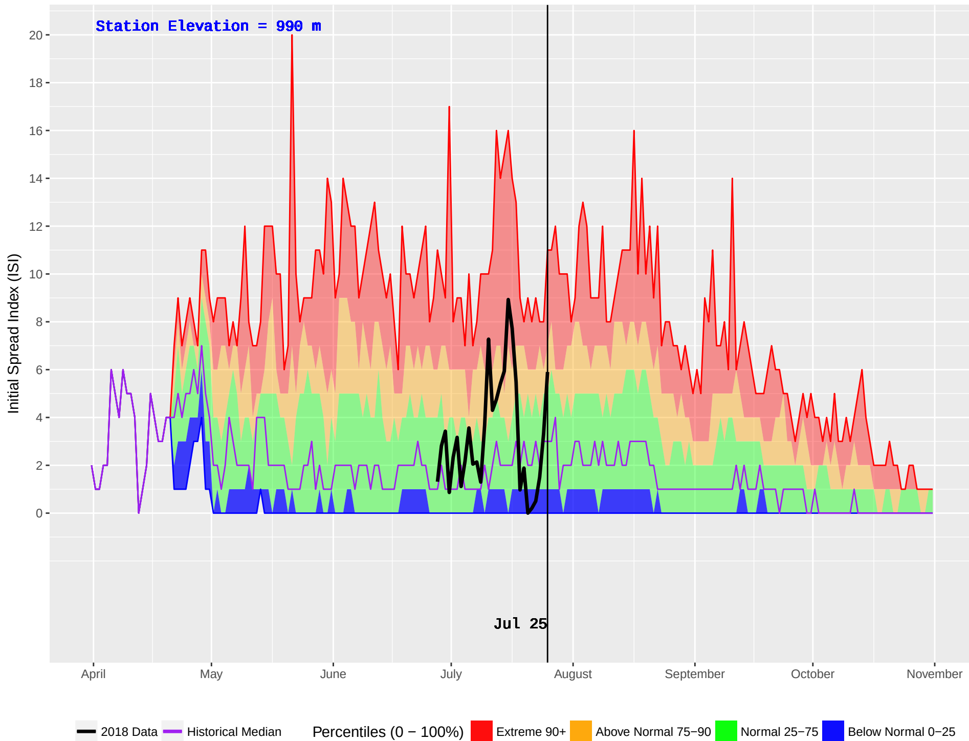
LOVELL COVE (163) : Historical (1979–2016) and Current (2018) Noon Initial Spread Index (ISI)
