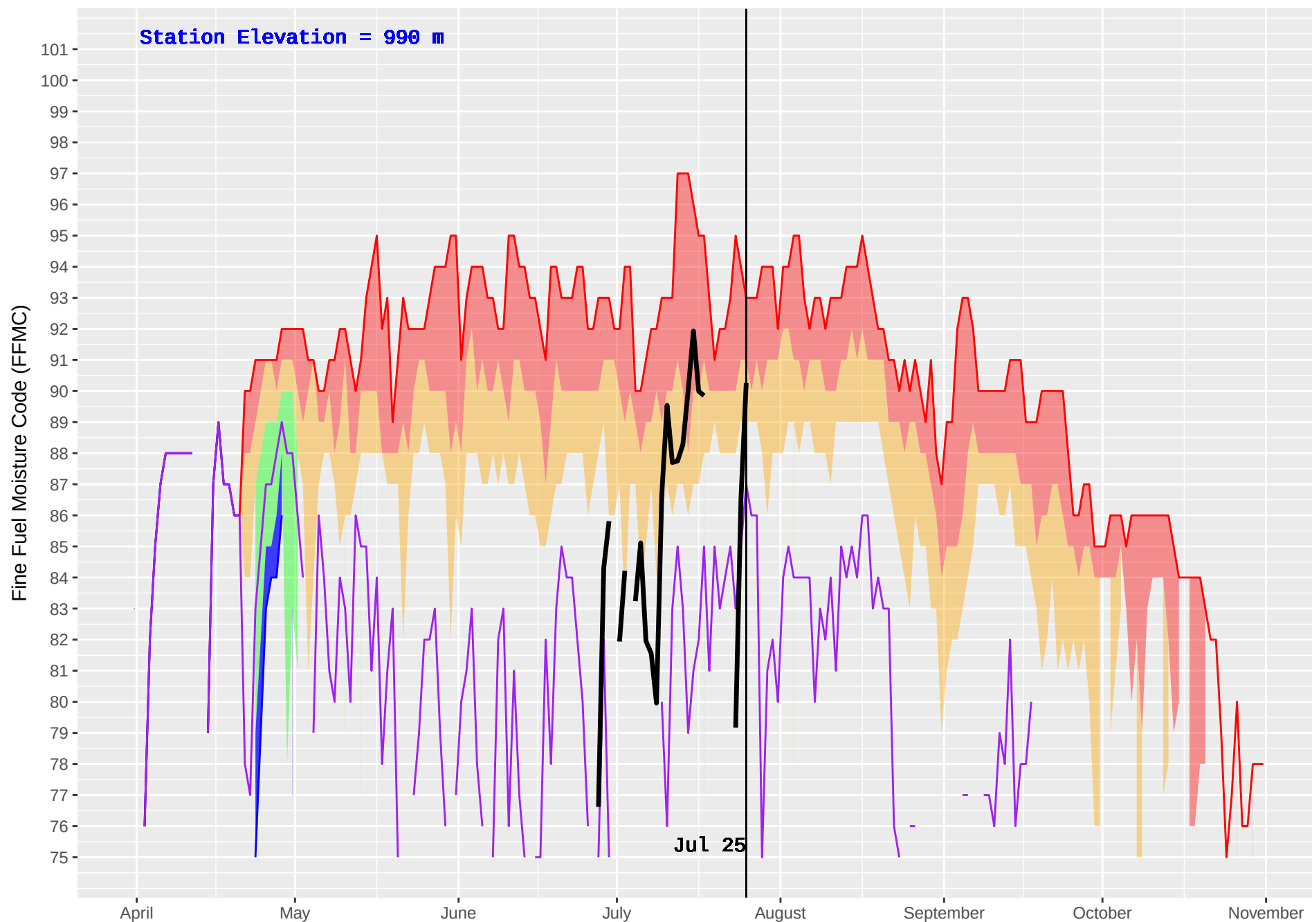
LOVELL COVE (163) : Historical (1979–2016) and Current (2018) Noon Fine Fuel Moisture Code (FFMC)
