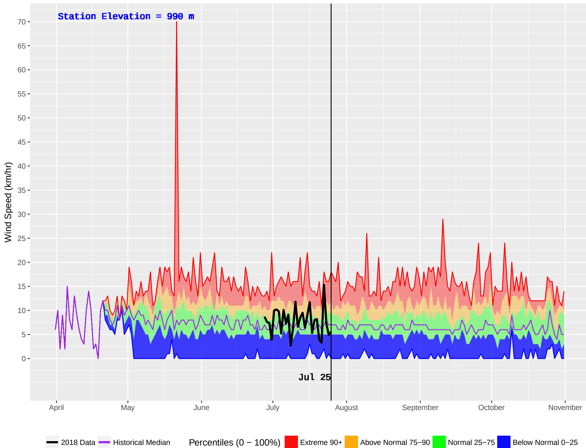
LOVELL COVE (163) : Historical (1979–2016) and Current (2018) Noon Wind Speed
