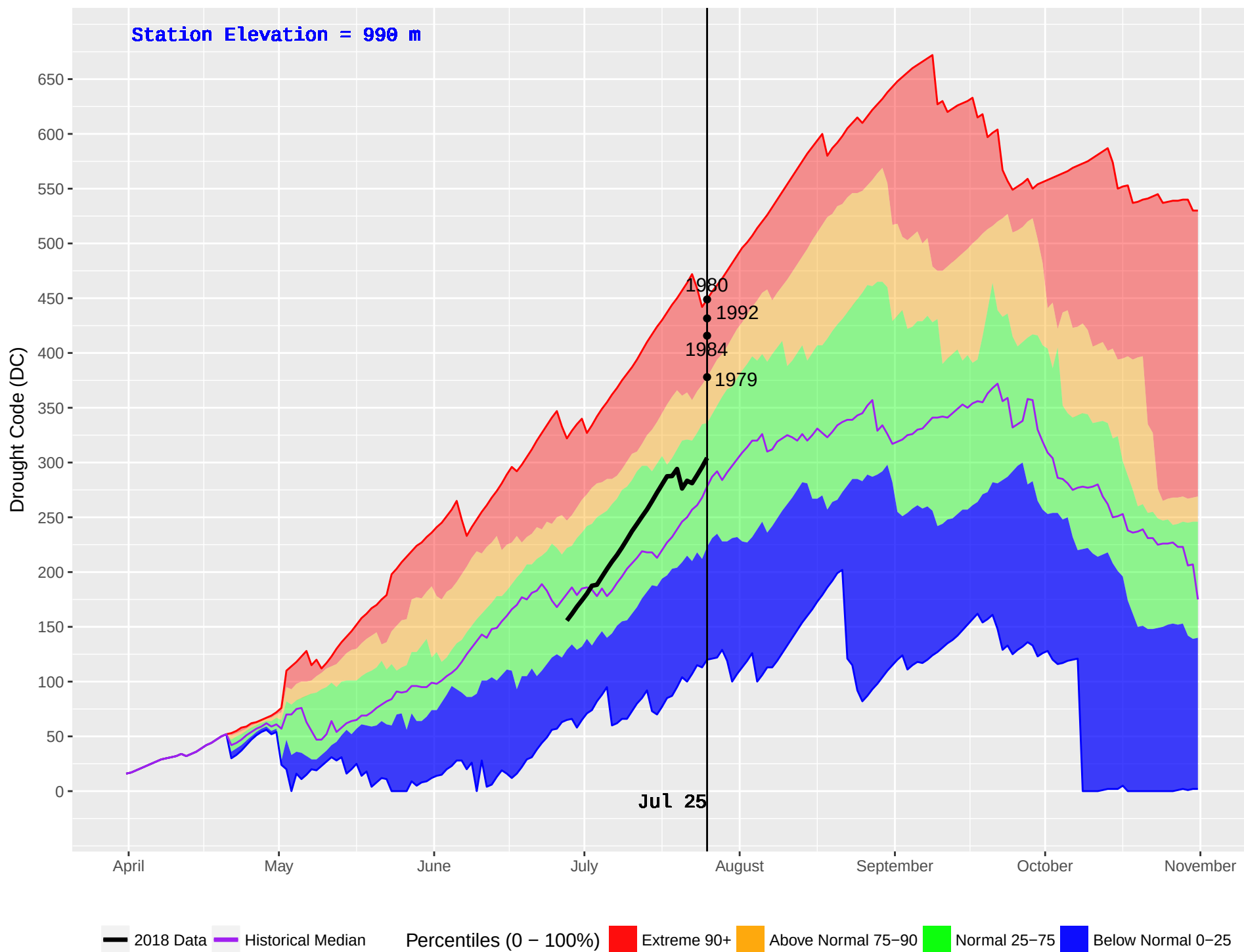
LOVELL COVE (163) : Historical (1979–2016) and Current (2018) Noon Drought Code (DC)
