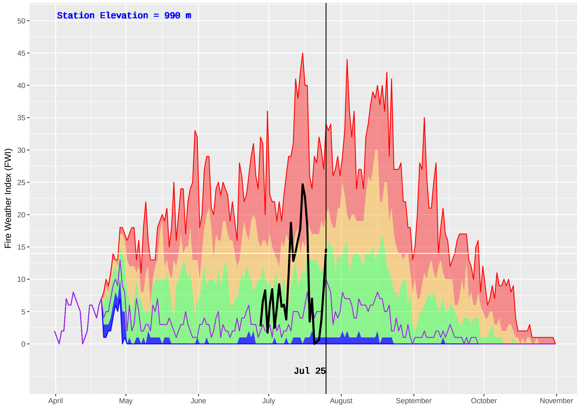
LOVELL COVE (163) : Historical (1979–2016) and Current (2018) Noon Fire Weather Index (FWI)
