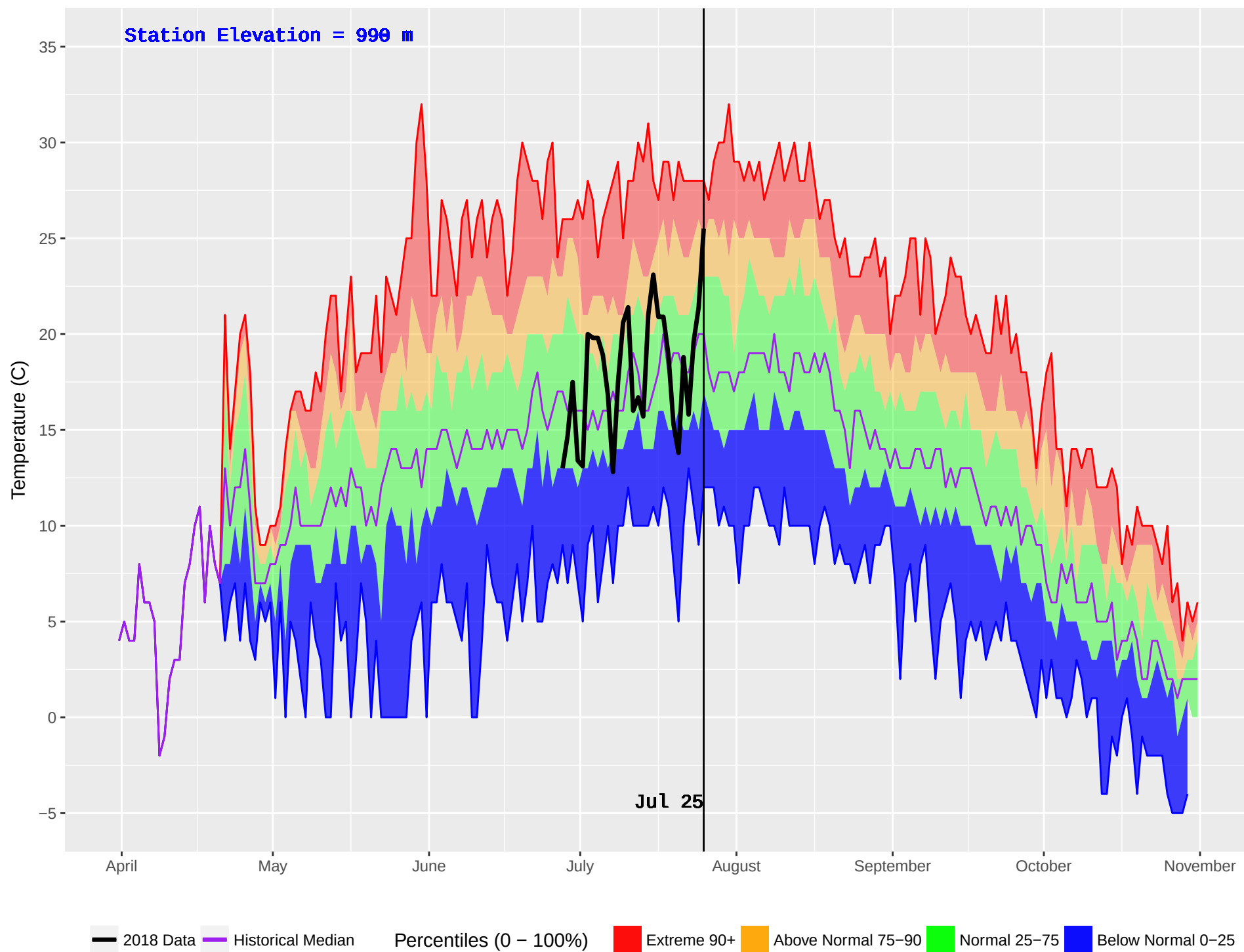
LOVELL COVE (163) : Historical (1979–2016) and Current (2018) Noon Temperature
