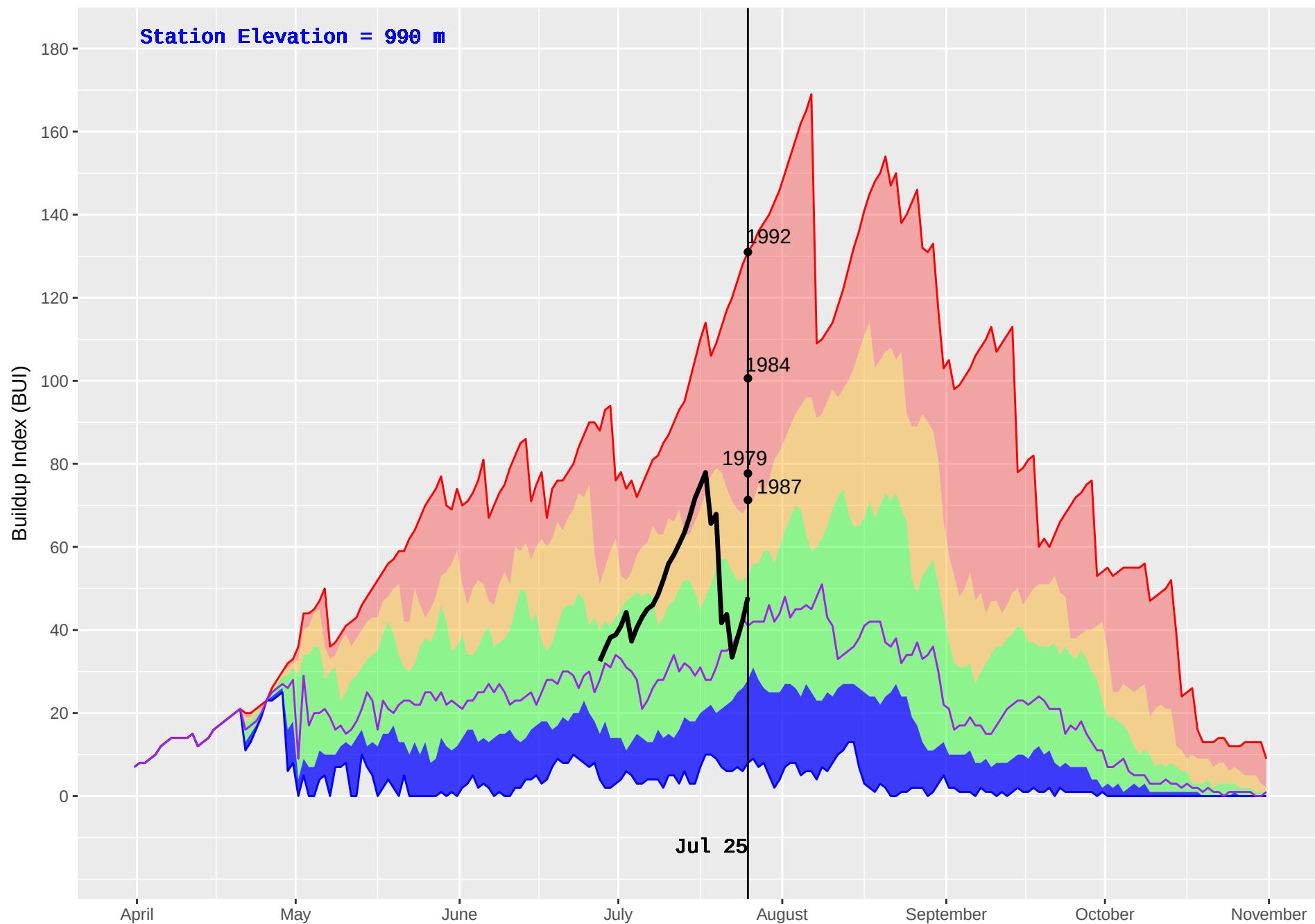
LOVELL COVE (163) : Historical (1979–2016) and Current (2018) Noon Buildup Index (BUI)
